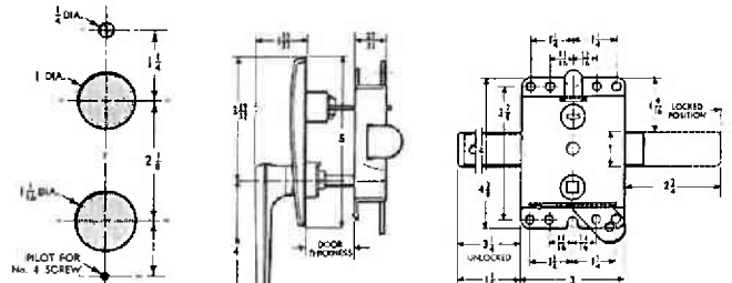
MOUNTING HOLES FOR HANDLE
